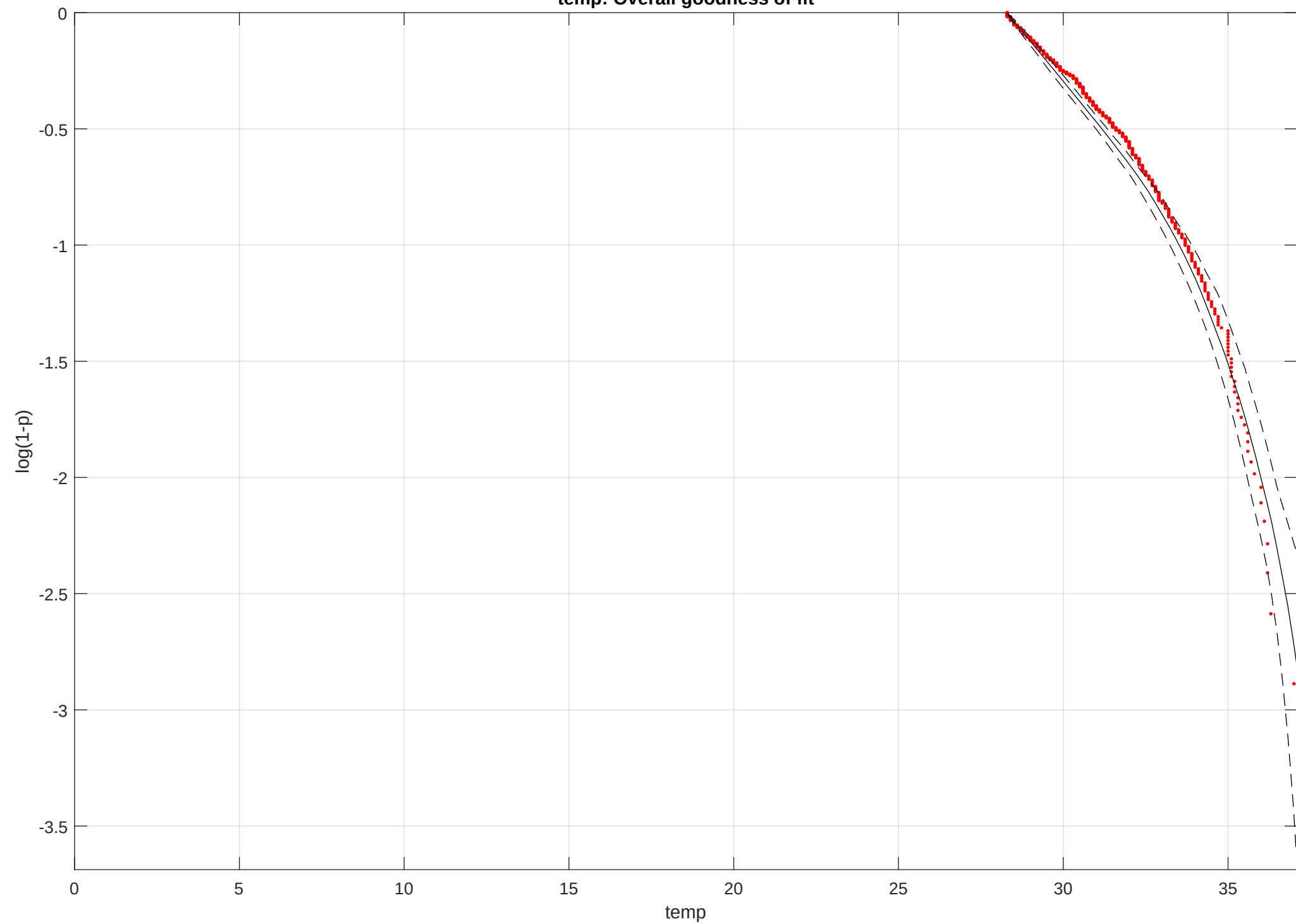
temp: Overall goodness of fit
